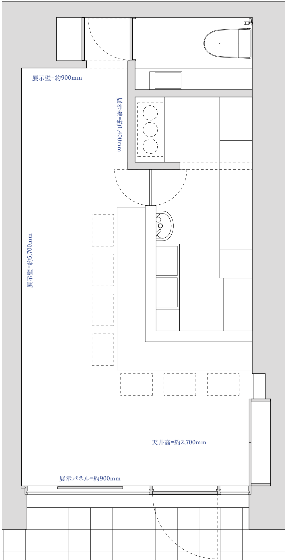
Gallery Café 3_plan_scale=1/30
